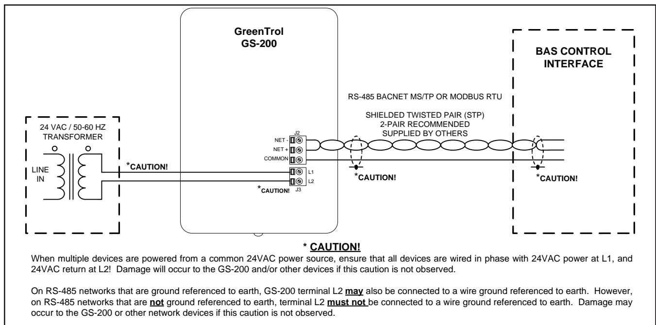
Figure 4. GS-200 Typical Wiring Diagram to BAS Control Interface
