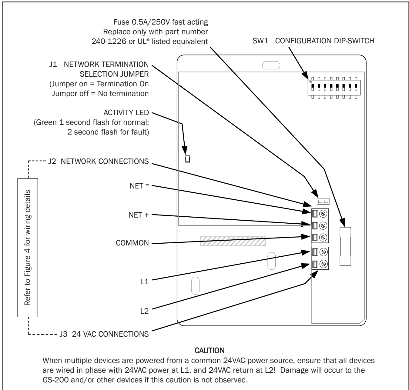
Figure 5. GS-200 Interior Detail View
